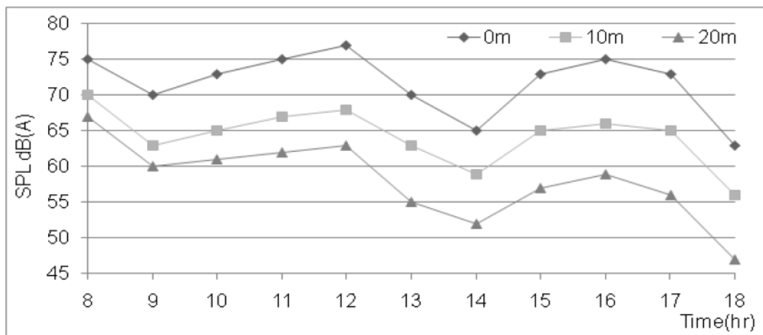
Fig. 7b. Variation of SPL for Barzani Namr Road at different distances
