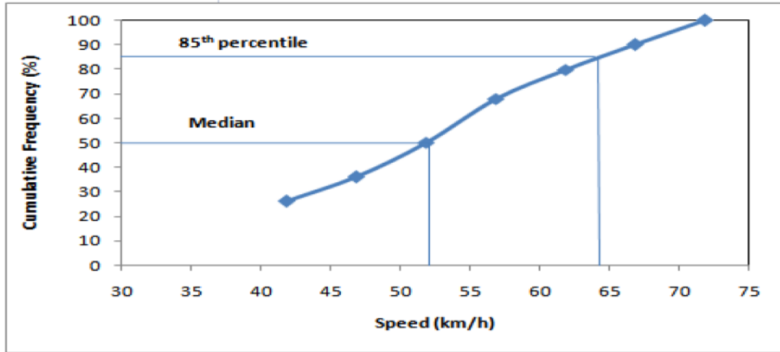
Fig. 4b. Cumulative distribution of spot speed data at Permatang Batu Road
