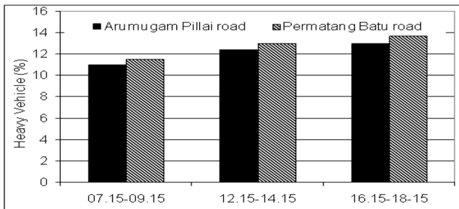
Fig.1d. Percent heavy vehicles for Arumugam Pillai and Permatang Batu Roads
