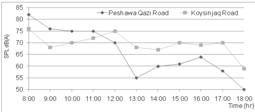
Fig. 6b. Variation of SPL for Peshawa Qazi and Koysinjaq Roads
