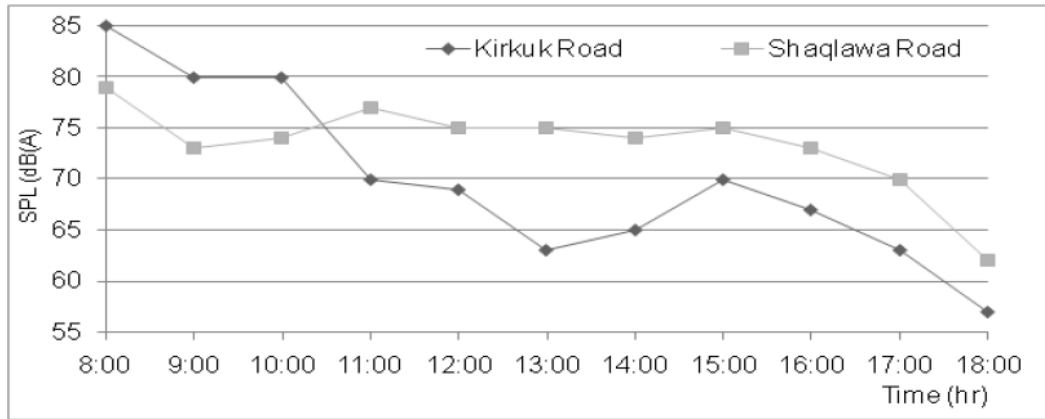
Fig. 6a. Variation of SPL for Kirkuk and Shaqlawa Roads
