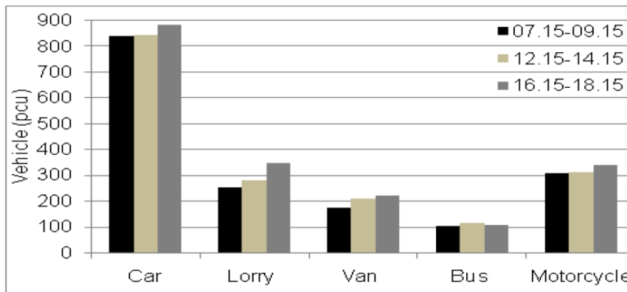
Fig. 1b. Traffic composition at Permatang Batu Road
