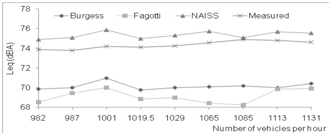
Fig. 5b. Leq comparison between different variants of traffic noise prediction model for Permatang Batu Road
