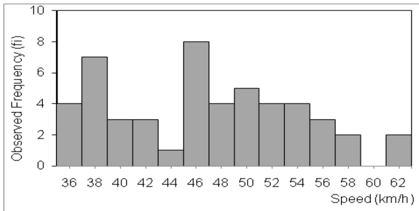
Fig. 3a. Histogram of spot speed data for Arumugam Pillai Road
