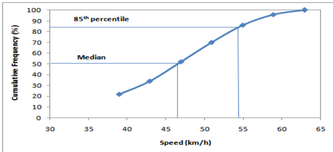
Fig. 4a. Cumulative distribution of spot speed data at Arumugam Pillai Road
