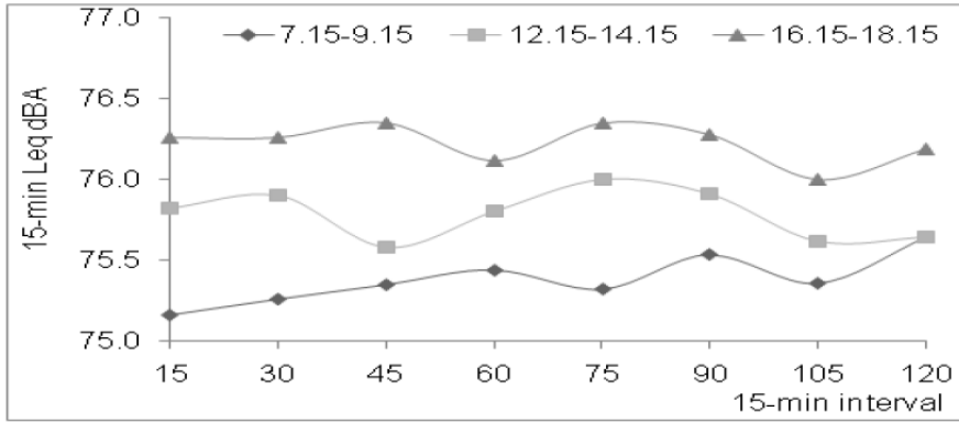
Fig. 2a. Trend noise level at Arumugam Pillai Road
