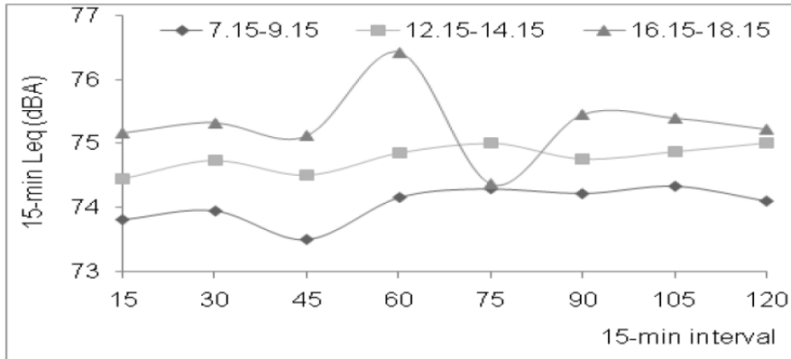
Fig. 2b. Trend noise level at Permatang Batu Road
