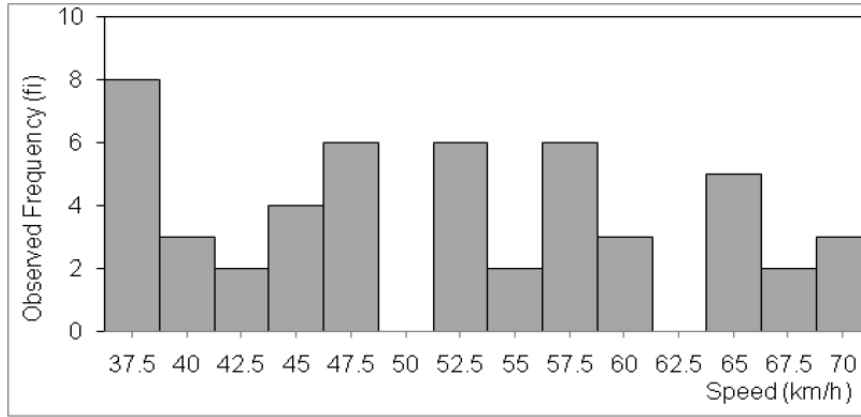
Fig. 3b. Histogram of spot speed data for Permatang Batu Road
