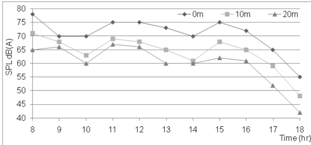
Fig. 7a. Variation of SPL for Kurdistan Road at different distances
