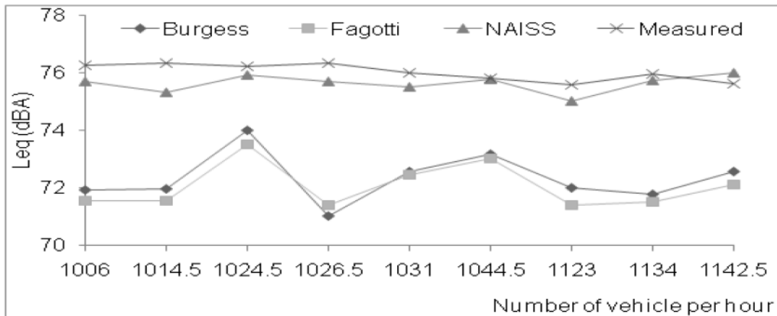
Fig. 5a. Leq comparison between different variants of traffic noise prediction model for Arumugam Pillai Road
